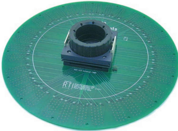
RTI BGA Universal Socket On Paragon Test Board 512
