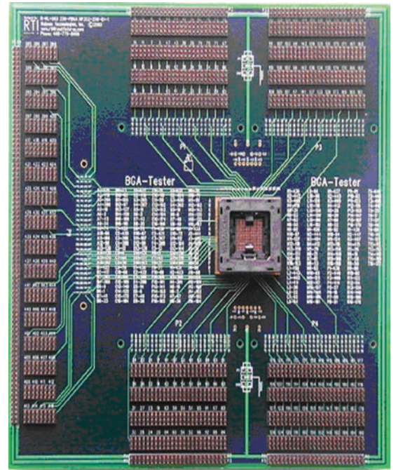
TS 512 Hilevel DUT Board For BGA Programming Matrix to Allow Any Tester Channel To Be Tied To GND or V+
