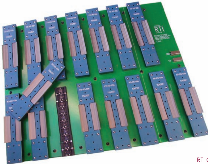
TS 512 Hilevel DUT Board For BGA Programming Matrix to Allow Any Tester Channel To Be Tied To GND or V+
