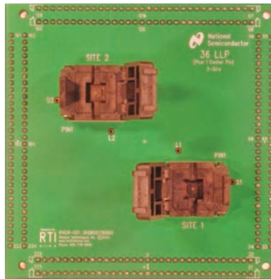
2 Site 256 Verifier Card
