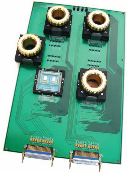
RTI Designed Burn-In Board With 4 Custom Sockets
