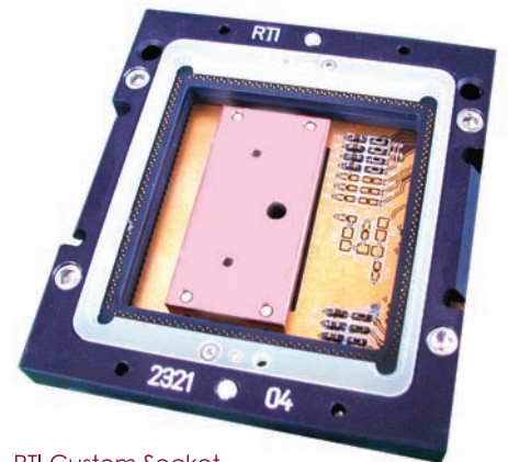
RTI Custom Socket. 300+ Pins, 0.5mm Pitch With Heat Sink
