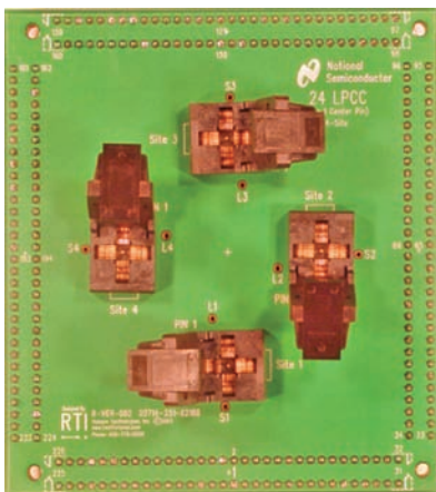
4 Site 256 Verifier Card
