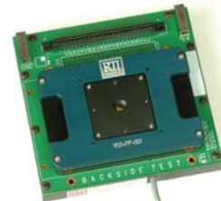
FA heated backside test fixture for QFN type packages
