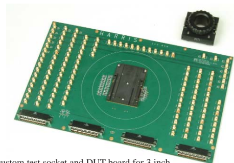
Full custom test socket and DUT board for 3 inch hybrid with 400 test pins on 0.8mm pitch
