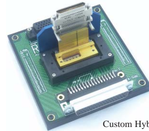
Custom Hybrid with 0.5 mm Pitch and Flex Circuit
