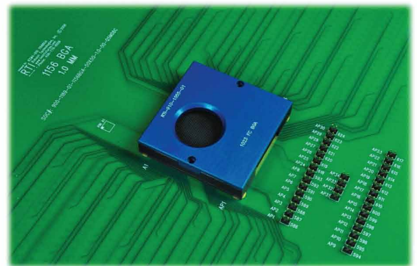
910-1055 Failure Analysis Lid
